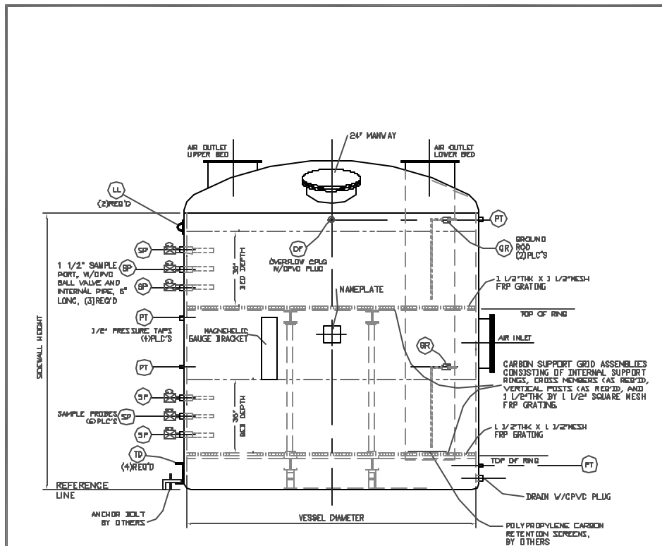
ELEVATION VIEW
