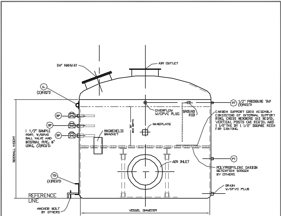
ELEVATION VIEW
